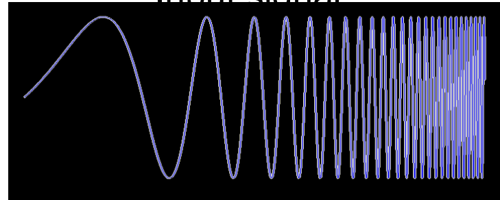
Matlab output:
