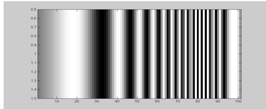
Matlab output:
