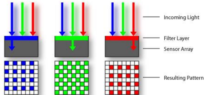
Bayer pattern
