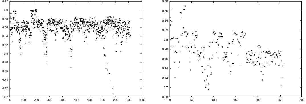
Figure 4: Rate of minimal DFA's with (k = 3, n = 7) for 915 slices and with (k = 2, n = 7) for 257 slices.
