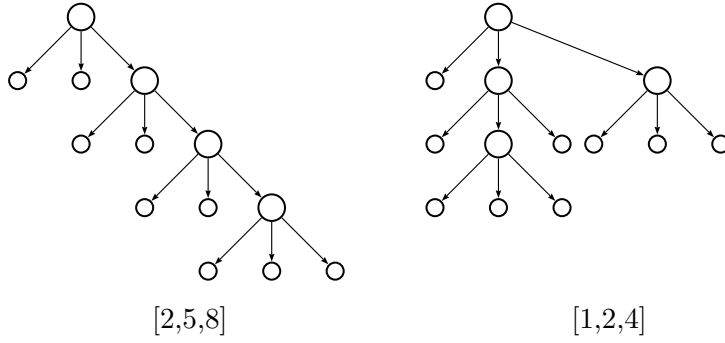
Figure 3: Two 3-ary trees with 4 internal nodes and the correspondent sequence of flags.
