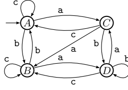
Figure 2: An ICDFFA 0 for which the string representation is [1, 2, 0, 2, 3, 0, 3, 0, 2, 1, 3, 2]
