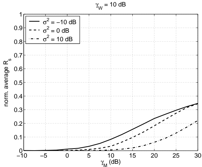
Fig. 12. Normalized average secure throughput versus \bar{\gamma}_M for \bar{\gamma}_W = 10 dB, and for selected values of \sigma^2 . Normalization is effected with respect to the capacity of an AWGN channel with SNR equal to \bar{\gamma}_M .
