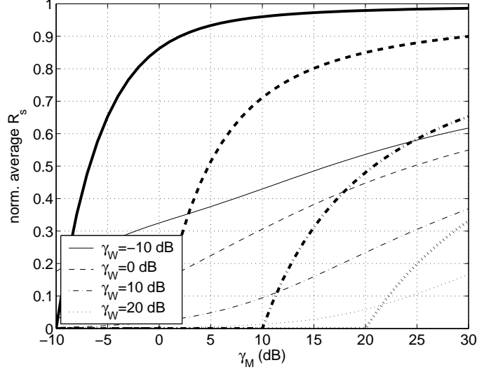
Fig. 10. Normalized average secrecy rate versus \bar{\gamma}_M , for selected values of \bar{\gamma}_W . Thinner lines correspond to the normalized average secrecy rate in the case of Rayleigh fading channels, while thicker lines correspond to the secrecy capacity of the Gaussian wiretap channel. Normalization is effected with respect to the capacity of an AWGN channel with SNR equal to \bar{\gamma}_M .
