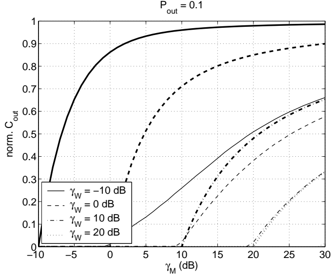
Fig. 6. Normalized outage secrecy capacity versus \bar{\gamma}_M , for selected values of \bar{\gamma}_W , and for an outage probability of 0.1. Thinner lines correspond to the normalized outage secrecy capacity in the case of Rayleigh fading channels, while thicker lines correspond to the secrecy capacity of the Gaussian wiretap channel. Normalization is effected with respect to the capacity of an AWGN channel with SNR equal to \bar{\gamma}_M .
