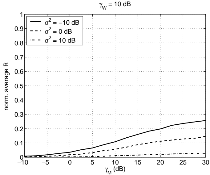
Fig. 13. Normalized average leaked throughput versus \bar{\gamma}_M for \bar{\gamma}_W = 10 dB, and for selected values of \sigma^2 . Normalization is effected with respect to the capacity of an AWGN channel with SNR equal to \bar{\gamma}_M .
