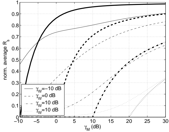
Fig. 14. Normalized average secrecy rate versus \bar{\gamma}_M , for selected values of \bar{\gamma}_W . Thinner lines correspond to the normalized average secrecy rate in the case of Rayleigh fading channels, while thicker lines correspond to the secrecy capacity of the Gaussian wiretap channel. Normalization is effected with respect to the capacity of an AWGN channel with SNR equal to \bar{\gamma}_M .
