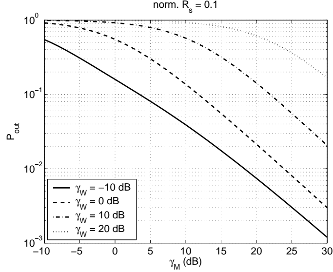
Fig. 4. Outage probability versus \bar{\gamma}_M , for selected values of \bar{\gamma}_W and for a normalized target secrecy rate equal to 0.1. Normalization is effected with respect to the capacity of an AWGN channel with SNR equal to \bar{\gamma}_M .
