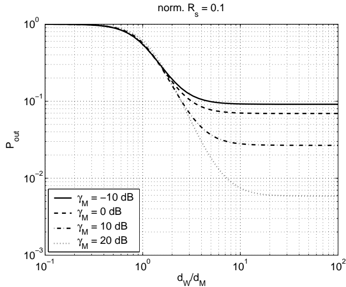
Fig. 5. Outage probability versus d_W/d_M , for selected values of \bar{\gamma}_M and for a normalized target secrecy rate equal to 0.1. Normalization is effected with respect to the capacity of an AWGN channel with SNR equal to \bar{\gamma}_M .
