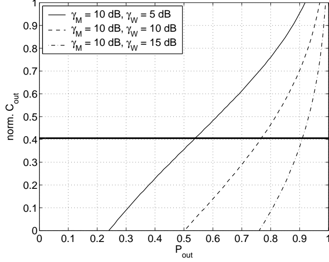
Fig. 8. Normalized outage secrecy capacity versus outage probability, for selected values of \bar{\gamma}_M and \bar{\gamma}_W . Thinner lines correspond to the normalized outage secrecy capacity of the eavesdropper's Rayleigh fading channel, while thicker lines correspond to the secrecy capacity of the Gaussian wiretap channel (in the last two cases this capacity is zero). Normalization is effected with respect to the capacity of an AWGN channel with SNR equal to \bar{\gamma}_M .
