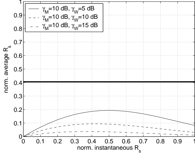
Fig. 9. Normalized average secrecy rate versus normalized instantaneous secrecy rate, for selected values of \bar{\gamma}_M and \bar{\gamma}_W . Thinner lines correspond to the normalized average secrecy rate of Rayleigh fading channels, while thicker lines correspond to the secrecy capacity of the Gaussian wiretap channel (in the last two cases this capacity is zero). Normalization is effected with respect to the capacity of an AWGN channel with SNR equal to \bar{\gamma}_M .
