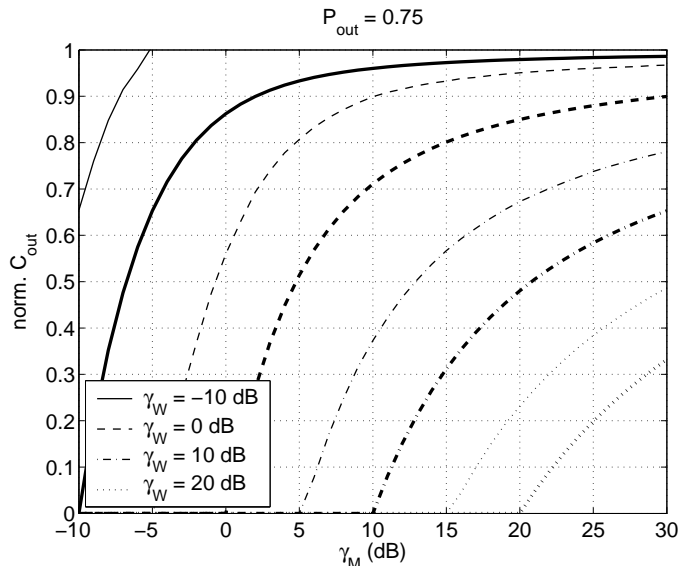
Fig. 7. Normalized outage secrecy capacity versus \bar{\gamma}_M , for selected values of \bar{\gamma}_W , and for an outage probability of 0.75. Thinner lines correspond to the normalized outage secrecy capacity in the case of the Rayleigh fading channels, while thicker lines correspond to the secrecy capacity of the Gaussian wiretap channel. Normalization is effected with respect to the capacity of an AWGN channel with SNR equal to \bar{\gamma}_M .
