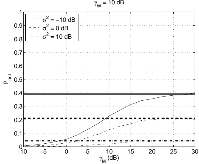
Fig. 11. Outage probability versus \bar{\gamma}_M for \bar{\gamma}_W = 10 dB, and for selected values of \sigma^2 . Thicker lines correspond to the upper bound to the outage probability while thinner lines correspond to the true outage probability.
