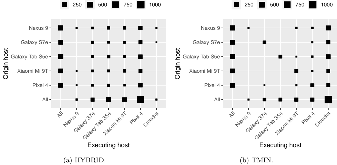
Figure 13: Cloudlet scenario – flow of jobs for \lambda = 12 and d = 9 (number of jobs).
