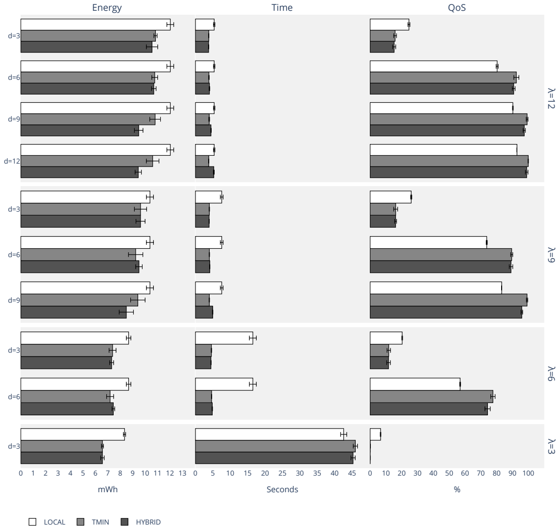
Figure 7: Android devices scenario – energy, time, and QoS.
