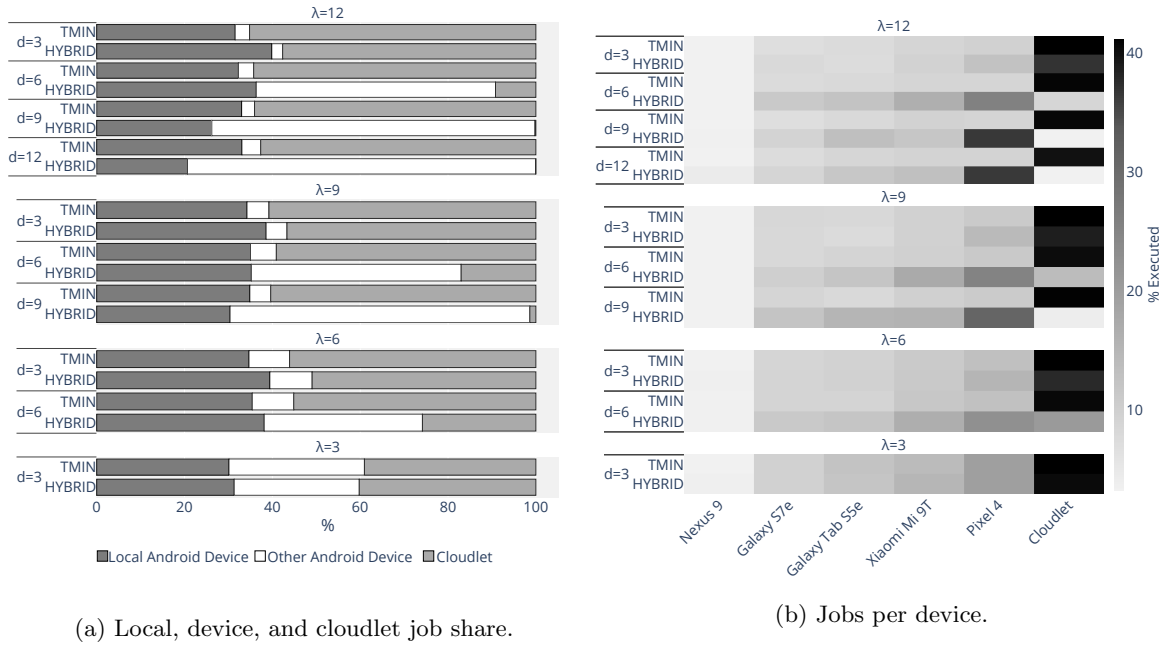
Figure 12: Cloudlet scenario – job distribution.
