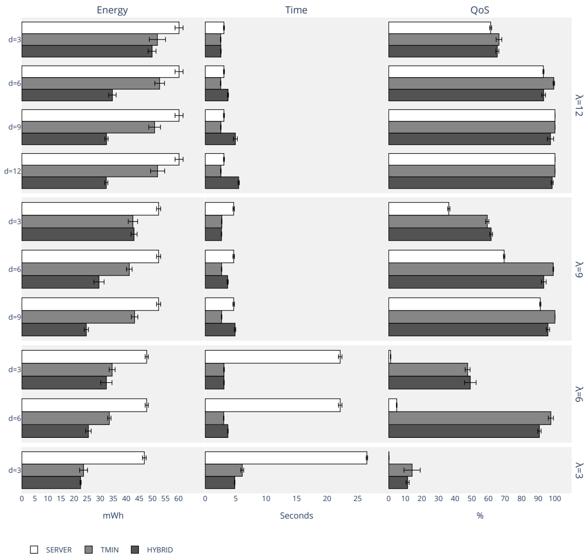
Figure 11: Cloudlet scenario – energy, time and QoS.
