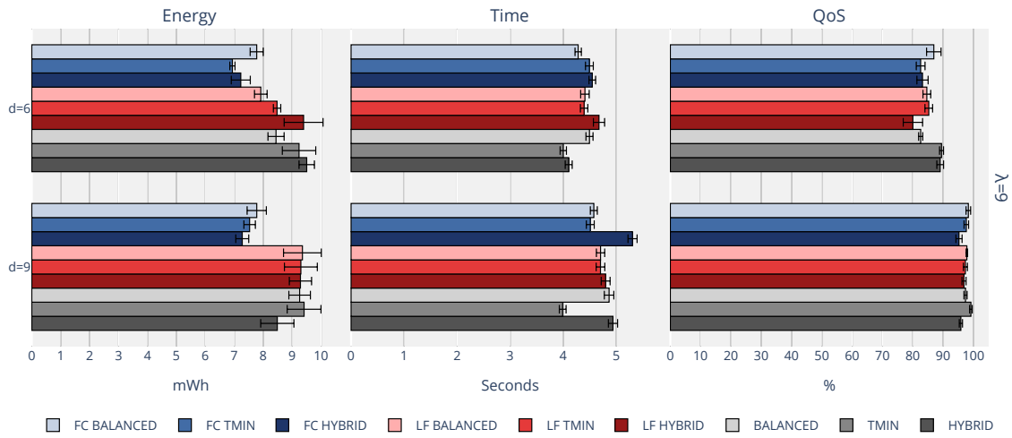
Figure 15: Additional scenarios – energy, time and QoS.
