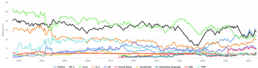
TIOBE Programming Community Index
