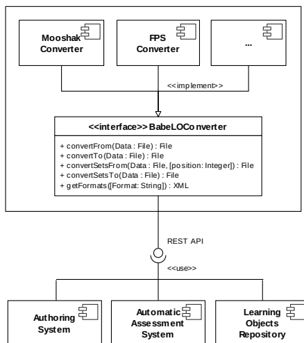
Fig. 2. BabelO architecture.
