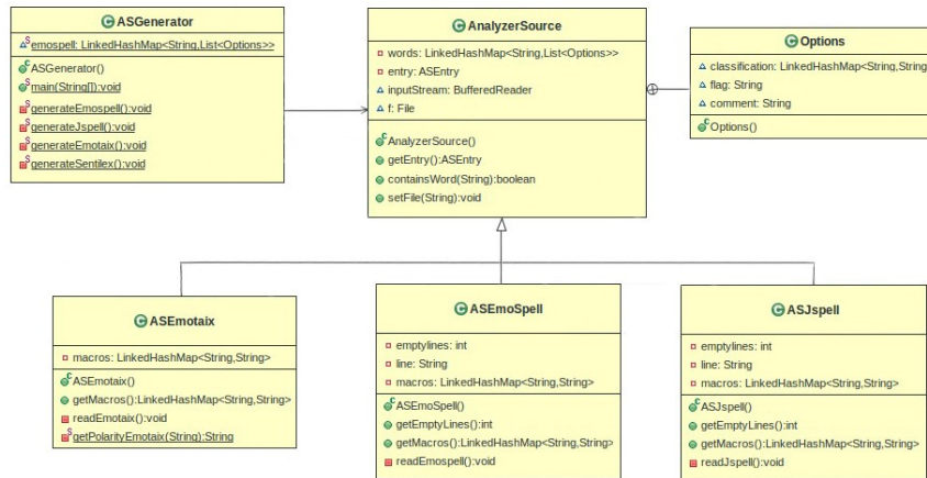
■ Figure 3 UML Diagram of of EmoSpell dictionary generator
